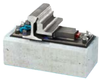
Inner Stock Rail Fastening
